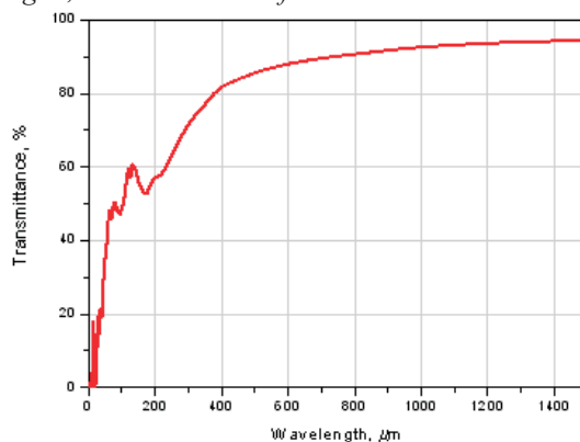
Fig. 1, 2 Transmission of LPF23.4.
