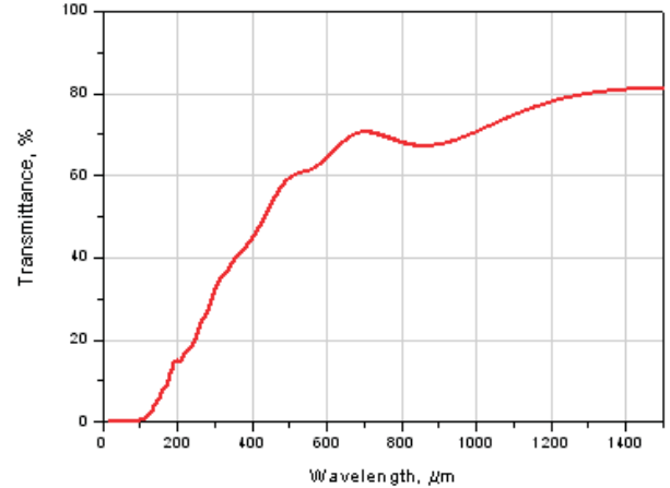
Fig. 17, 18 Transmission of LPF4.0.
