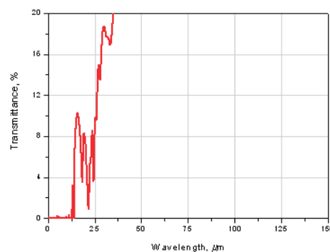
Fig. 1, 2 Transmission of LPF23.4.
