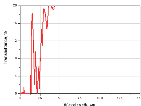
Fig. 3, 4 Transmission of LPF23.3.
