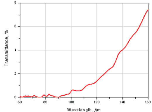
Fig. 19, 20 Transmission of LPF3.2.
